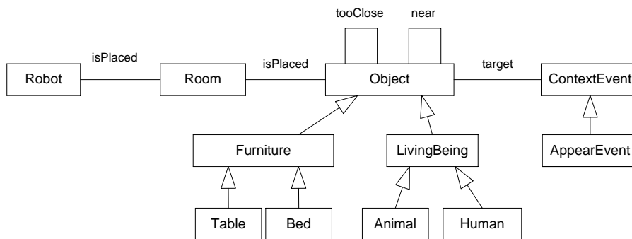
Fig. 2. Part of a context metamodel
