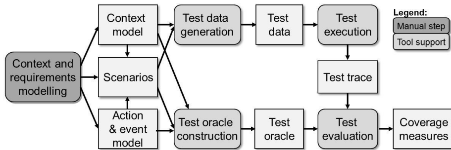
Fig. 1. Overview of the testing framework
