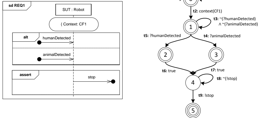
Fig. 5. Observer automaton generated from the scenario
